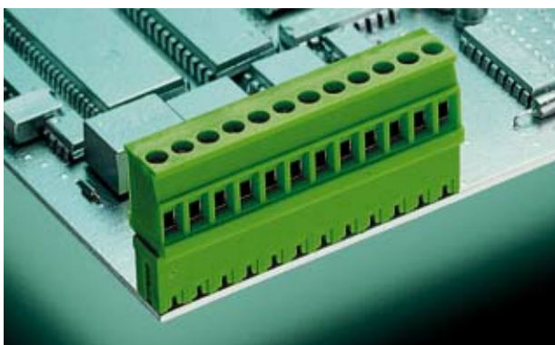
AK(Z) 1110/.. - 5,0 (5,08) - green
